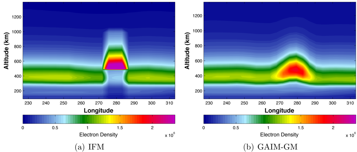
Figure 34. GAIM-GM electron density reproduction of the high altitude synthetic SED, using the AFWA+100 grid at 1945 UT. Both latitude slices were taken at 40° N. Note how GAIM-GM did not accurately capture the vertical profile of the SED
